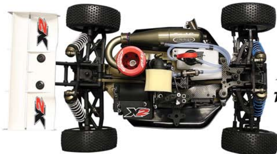
Engine Mounts - hard anodized billet aluminum, easily adjustable with cooling fins.
